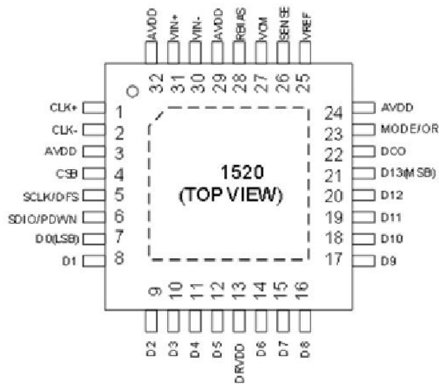
QFN5X5-32
