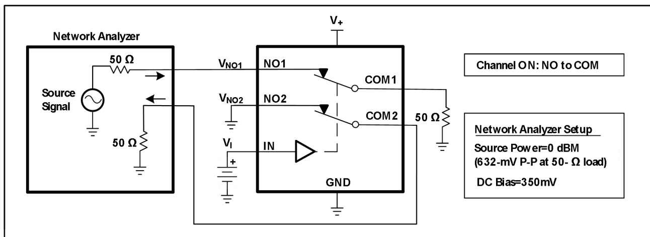
图 12. 串扰 (X TALK )
