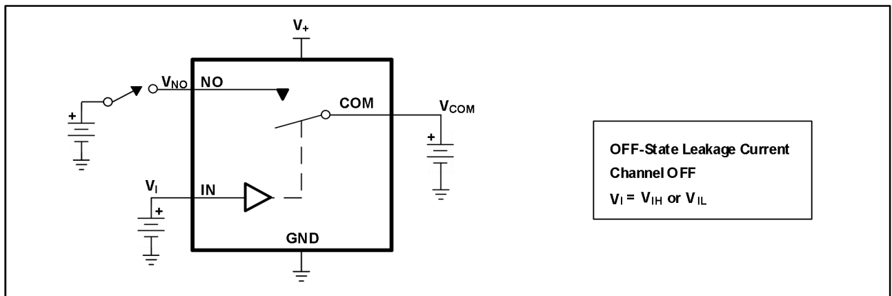
图 5. OFF 状态漏电流 ( I_{COM(OFF)} , I_{NO(OFF)} )
