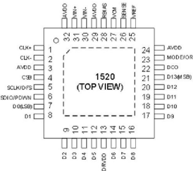
QFN5X5-32
