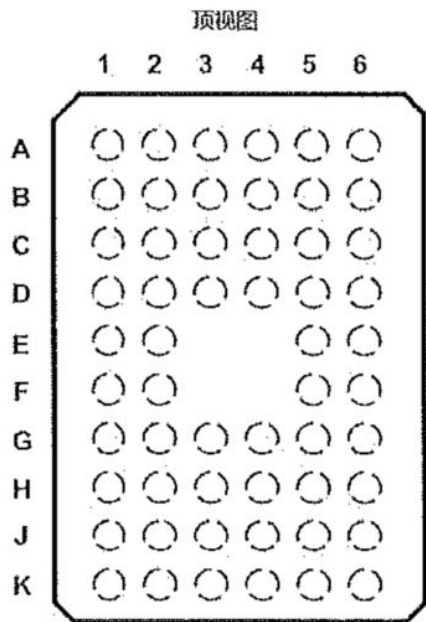
BGA56
