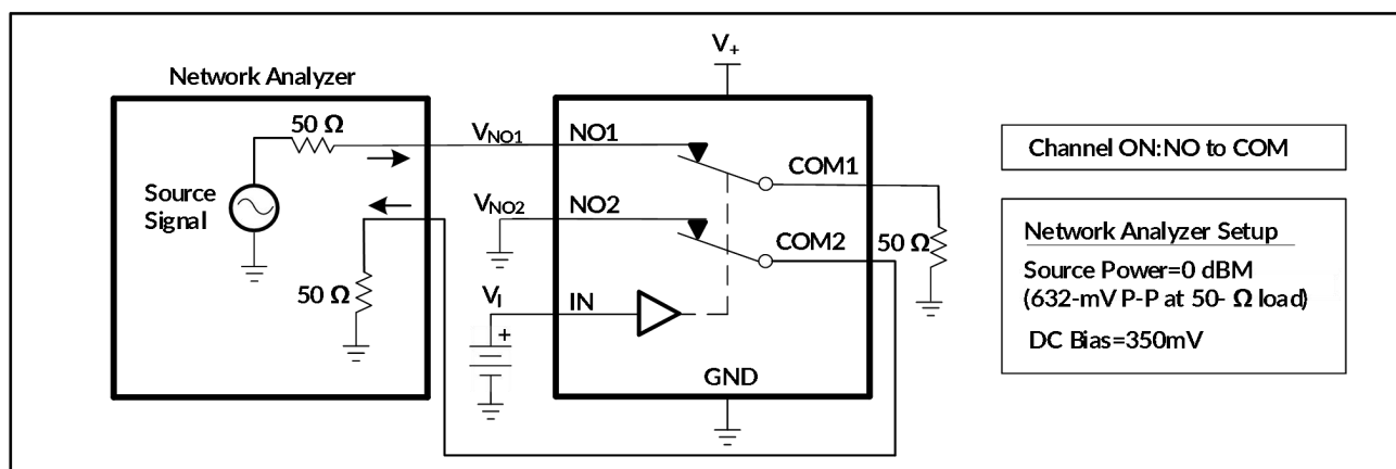
图 18. 串扰 (X TALK )
