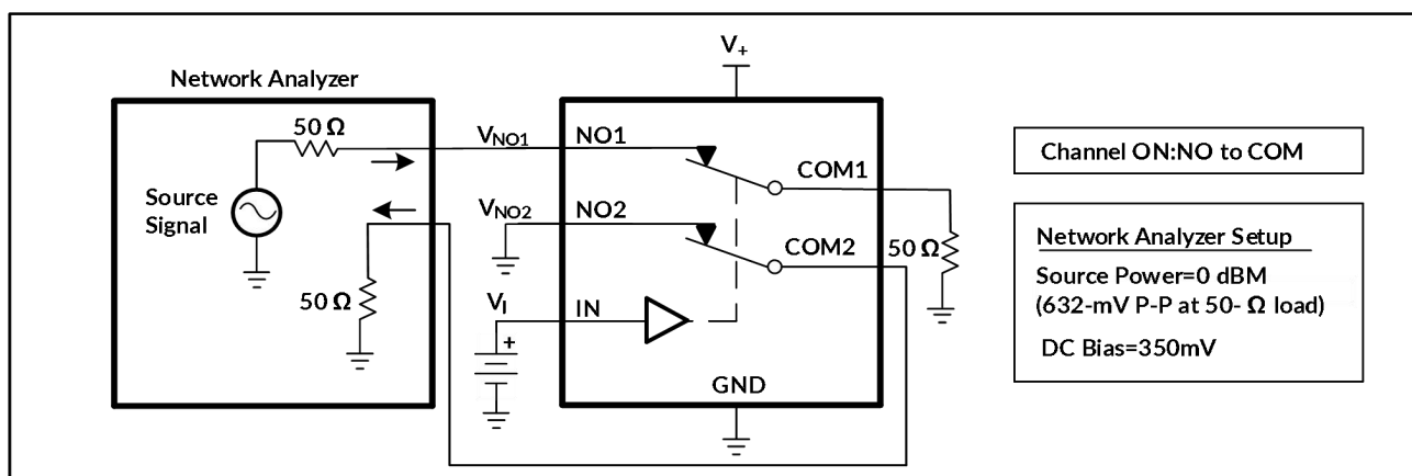
图 12. 串扰 (X TALK)
