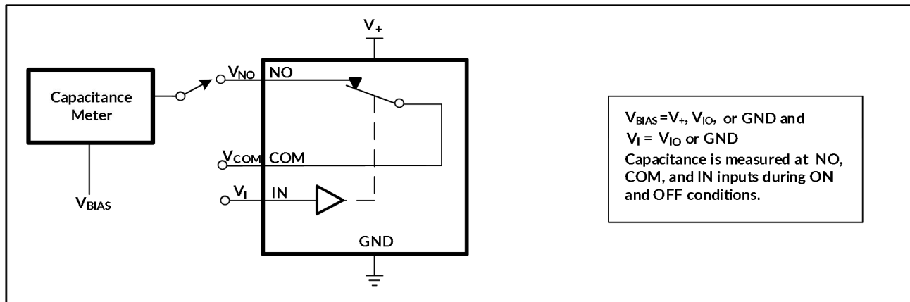
图 7. 电容 ( C_I , C_{COM(OFF)} , C_{COM(ON)} , C_{NO(OFF)} , C_{NO(ON)} )
