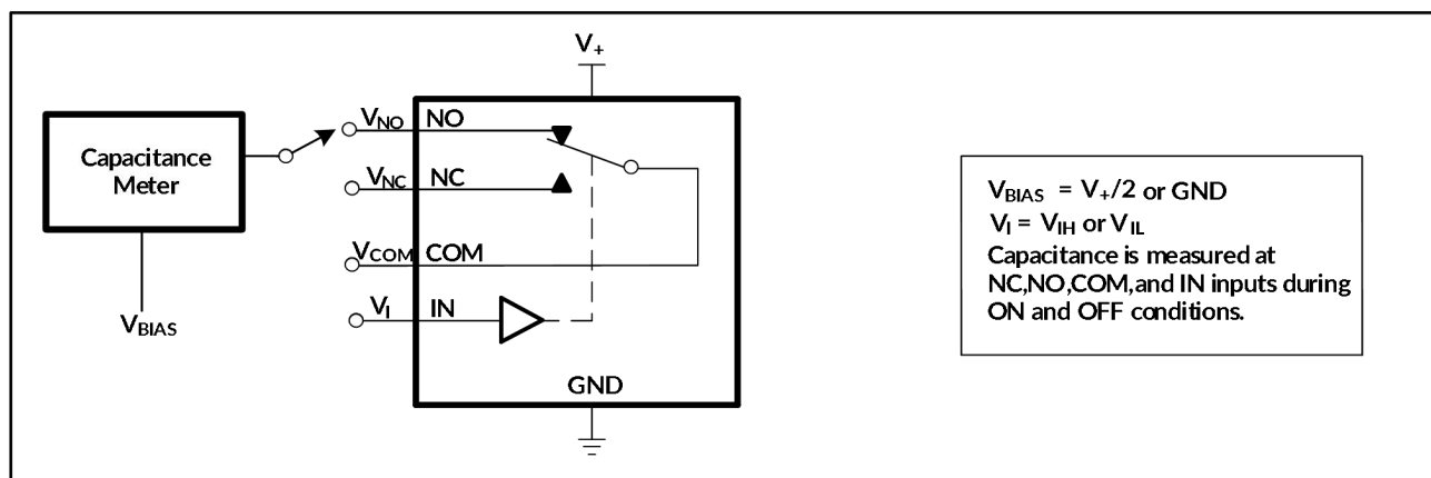
图 7. 电容 ( C_I , C_{COM(ON)} , C_{NC(OFF)} , C_{NC(ON)} , C_{NO(OFF)} , C_{NO(ON)} )
