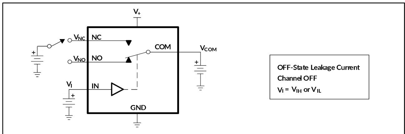
图 5. 关断漏电流 ( I_{NC(OFF)} , I_{NO(OFF)} )
