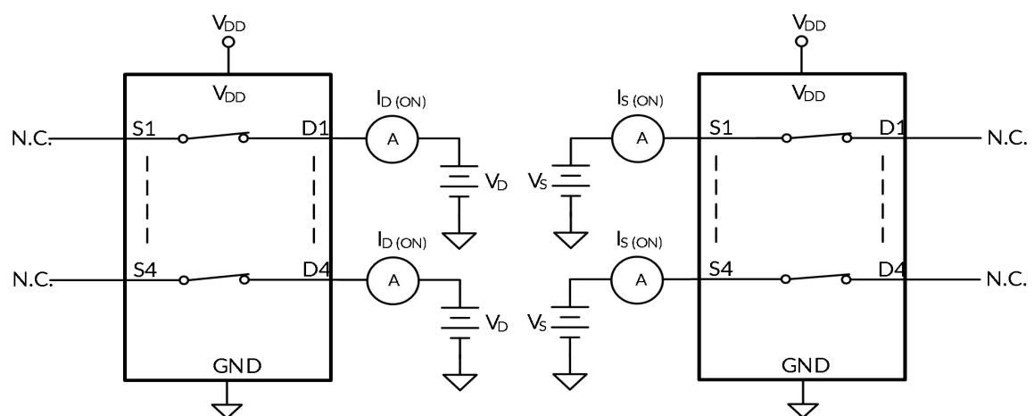
图 5. 关断漏电流 ( I_{D(OFF)} , I_{S(OFF)} )
