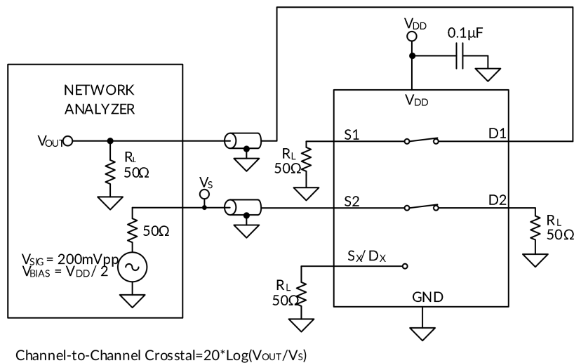
图 10. 串扰 (XTALK)
