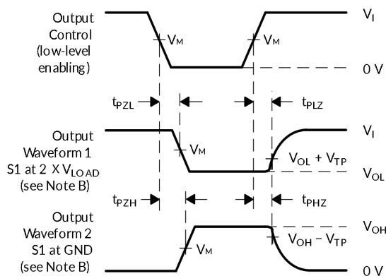
VOLTAGE WAVEFORMS ENABLE AND DISABLE TIMES
